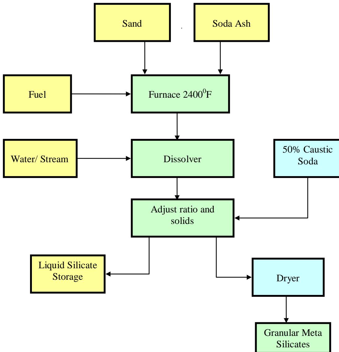
Figure 3.5 Production of sodium silicate
