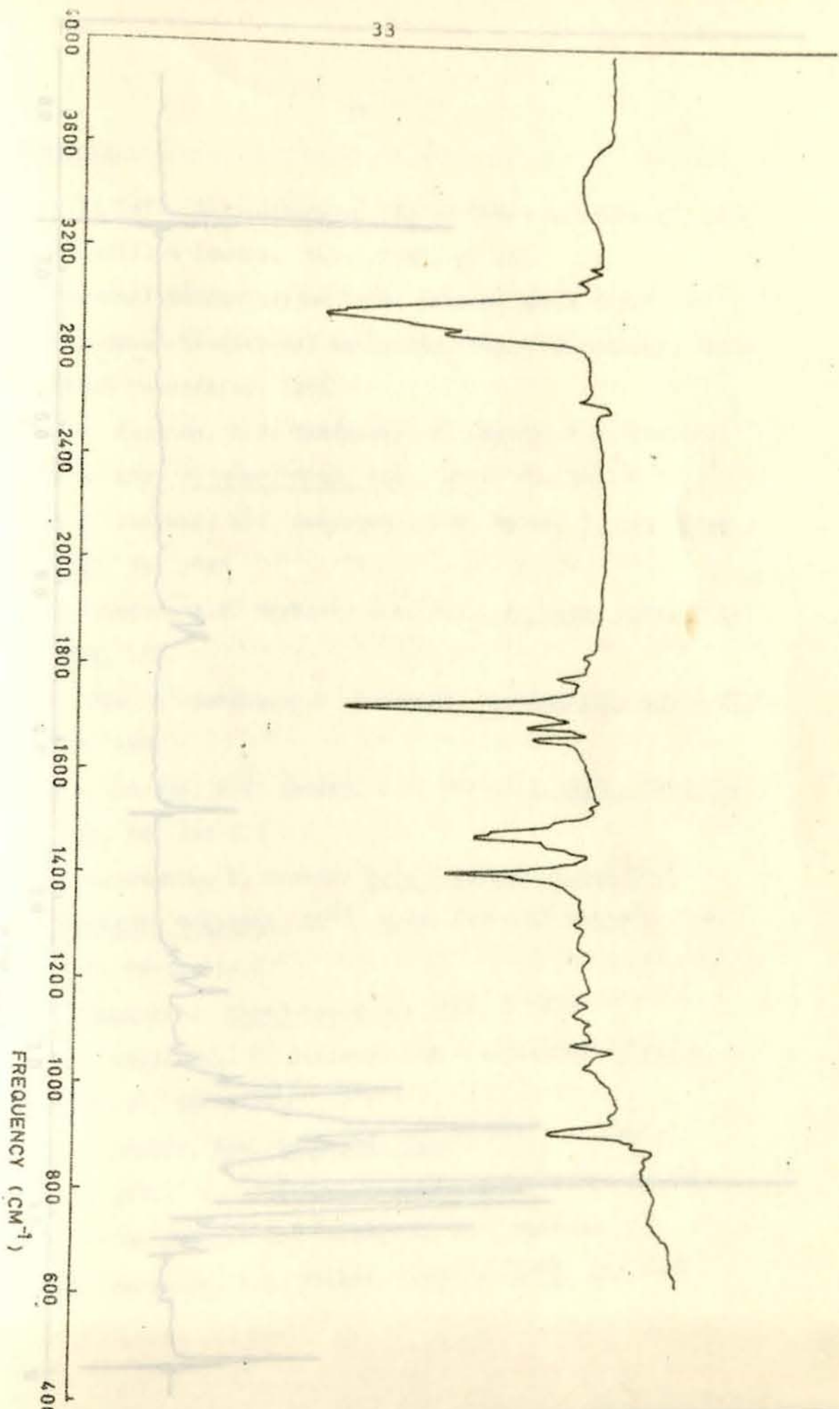
INFRARED SPECTRUM OF A2 CRYSTALS (KBr)
