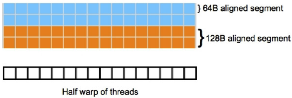
FIGURE 3.3: Linear Memory Segments and half of work-items per wavefront (warp in CUDA) [49]
