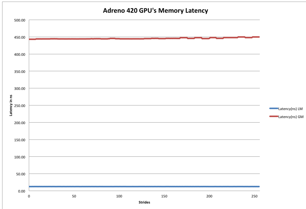
FIGURE 3.11: Read latency for the global and local memories of the Adreno 420 GPU
