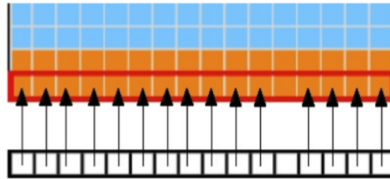
FIGURE 3.4: Coalesced Access: All work items except one access memory. One 64-byte segment is read from memory. [49]
