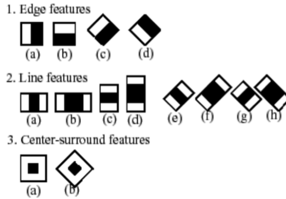
FIGURE 2.5: Haar-like features (Reproduced from[17])
