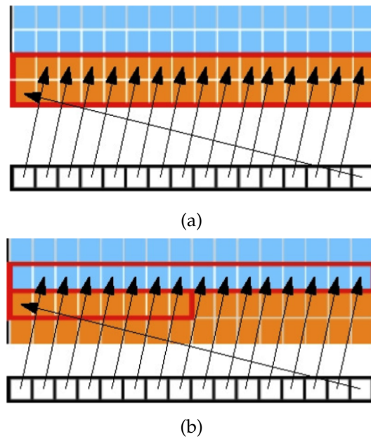
FIGURE 3.5: Misaligned Sequential Memory Access [49]
