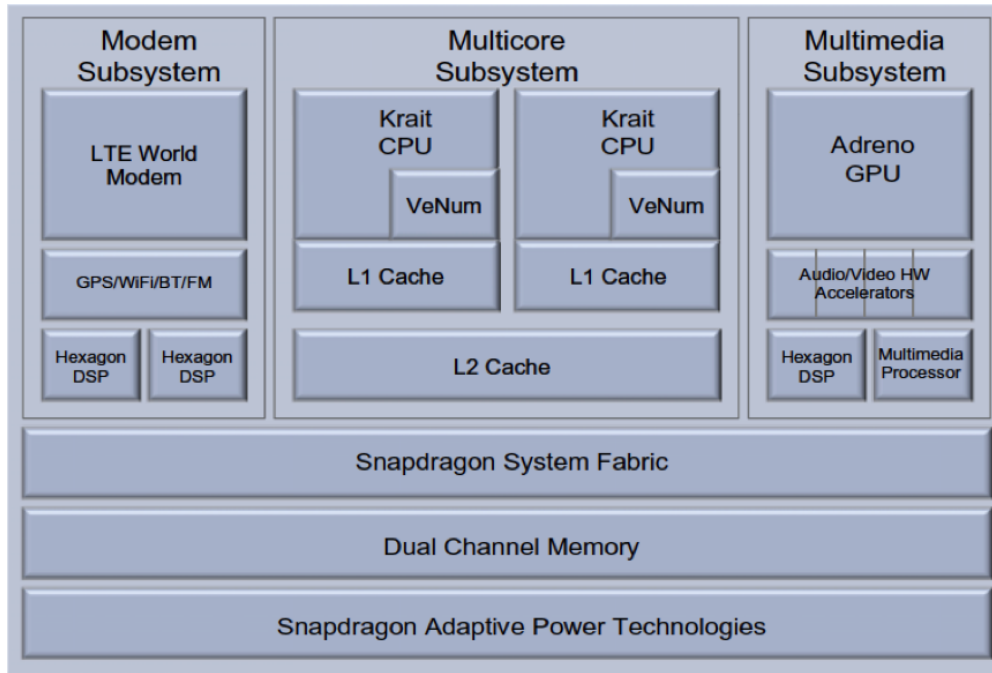
FIGURE 3.1: Architecture of dual core Qualcomm Snapdragon S4 Pro (MSM8960) [23]
