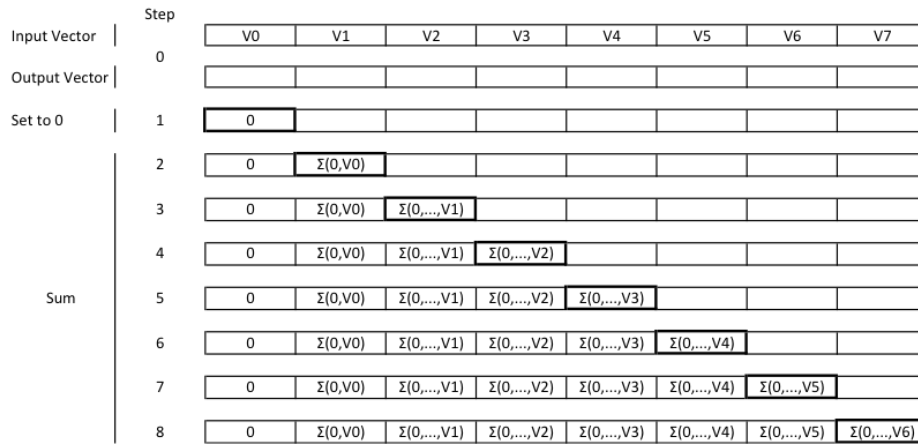
FIGURE 4.1: Sequential computing of an exclusive prefix sum (scan)
