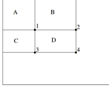
FIGURE 2.8: Integral Image Representation Example (Reproduced from[17])
