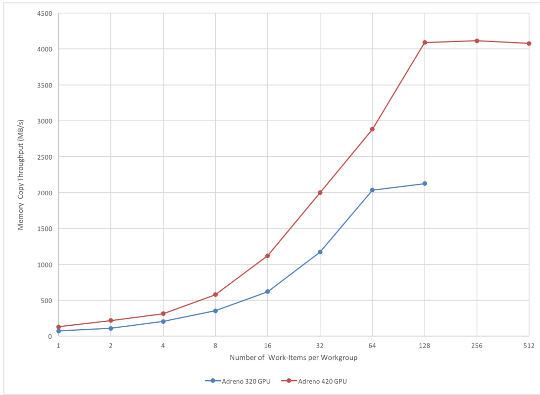
FIGURE 3.7: Coalesced Memory Access
