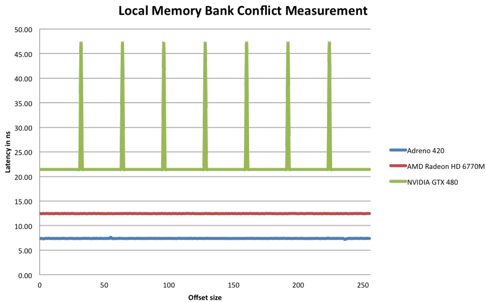
FIGURE 3.12: Local Memory Bank Conflict Measurement
