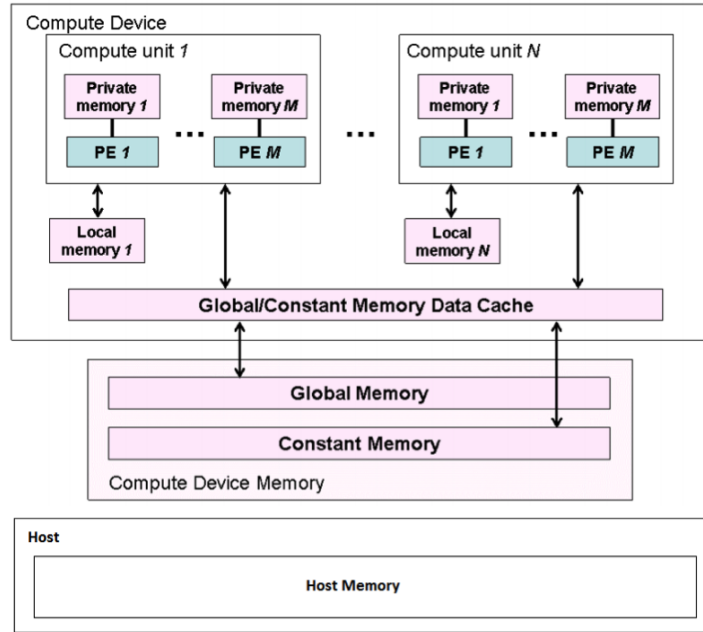
FIGURE 2.2: OpenCL Memory Model (Reproduced from[32])
