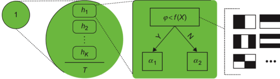
FIGURE 2.6: One stage of the cascade classifier in OpenCV (Reproduced from [17])
