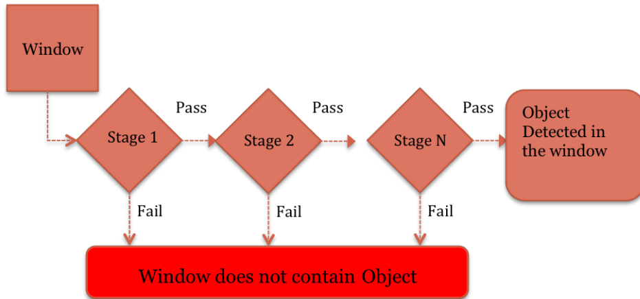
FIGURE 2.4: The Cascade Classifier Process
