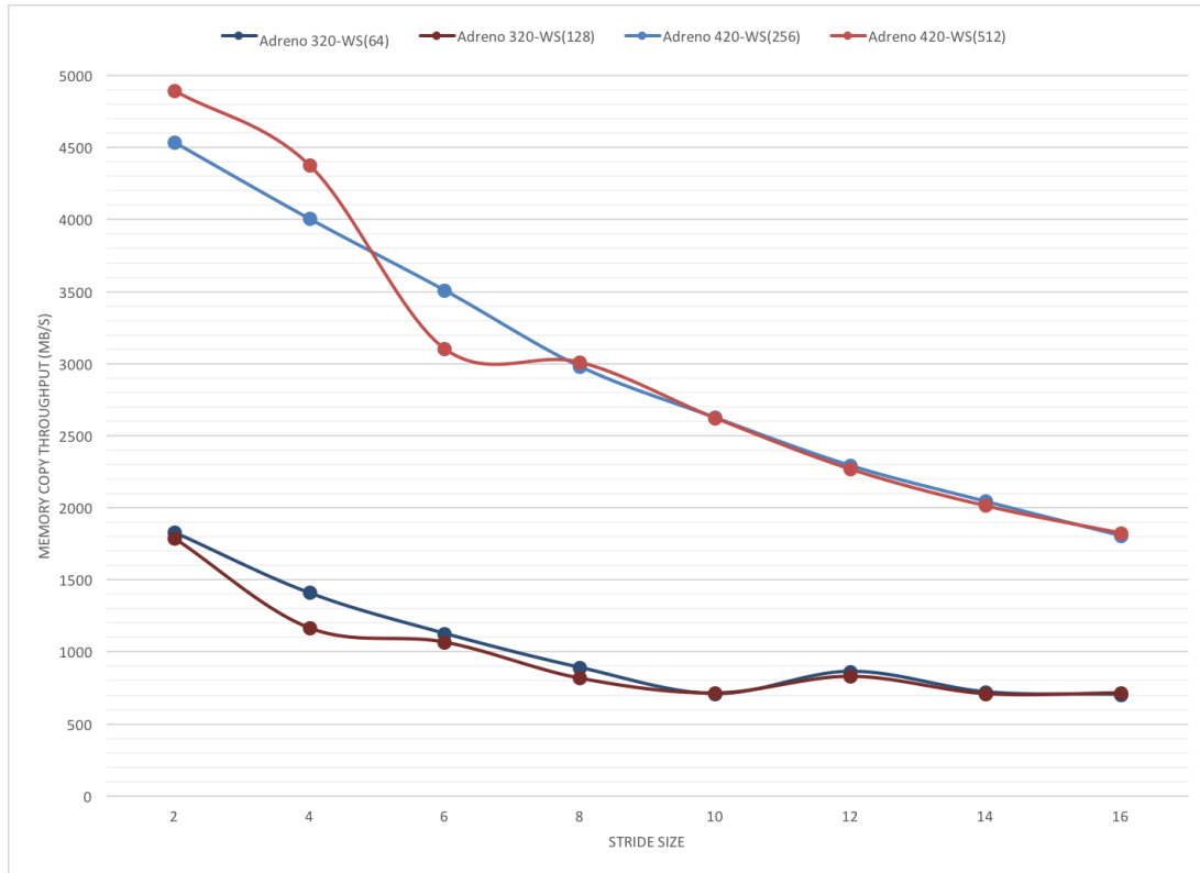
FIGURE 3.9: Global Memory Access with strides
