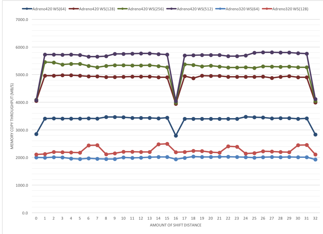
FIGURE 3.8: Global Memory Access with shifts
