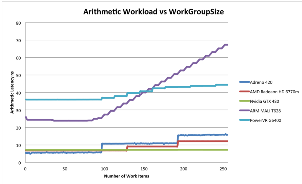
FIGURE 3.13: Arithmetic workload vs work-group-size
