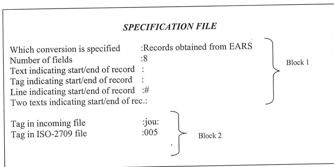
Figure 4.6. Partial Conversion Specification File for EARS output
