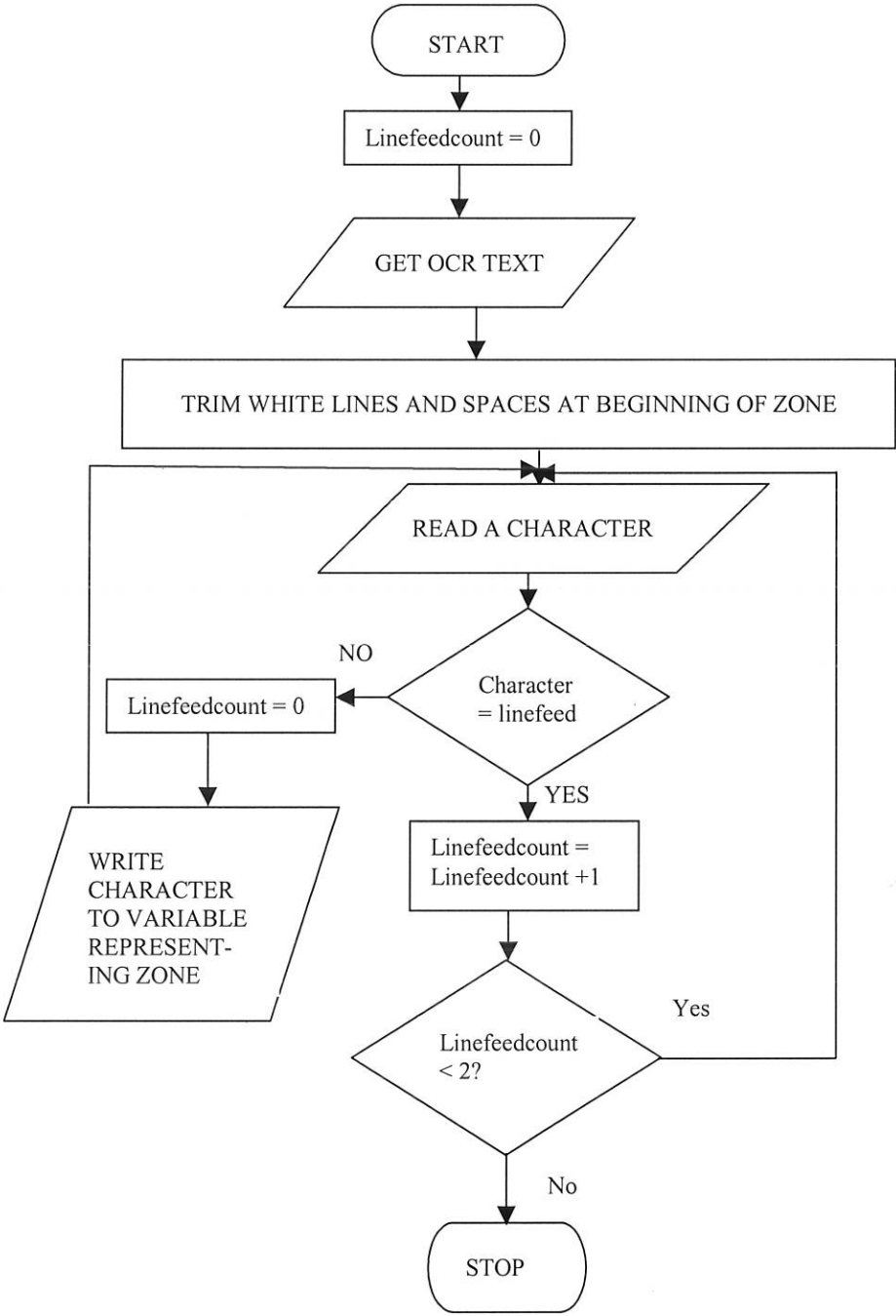
Figure 4.3. Flowchart for the first level segmentation algorithm
