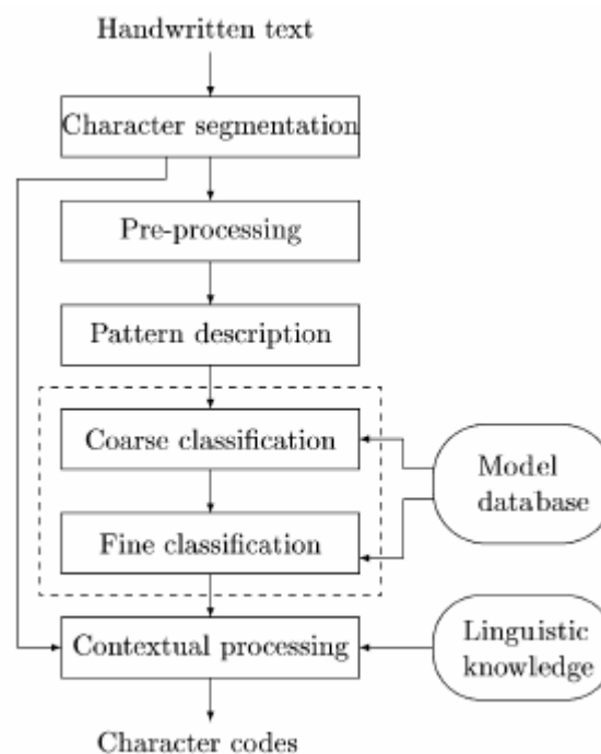
Figure 3.2 Diagram of a practical online Chinese character recognition system (OLCCR)
