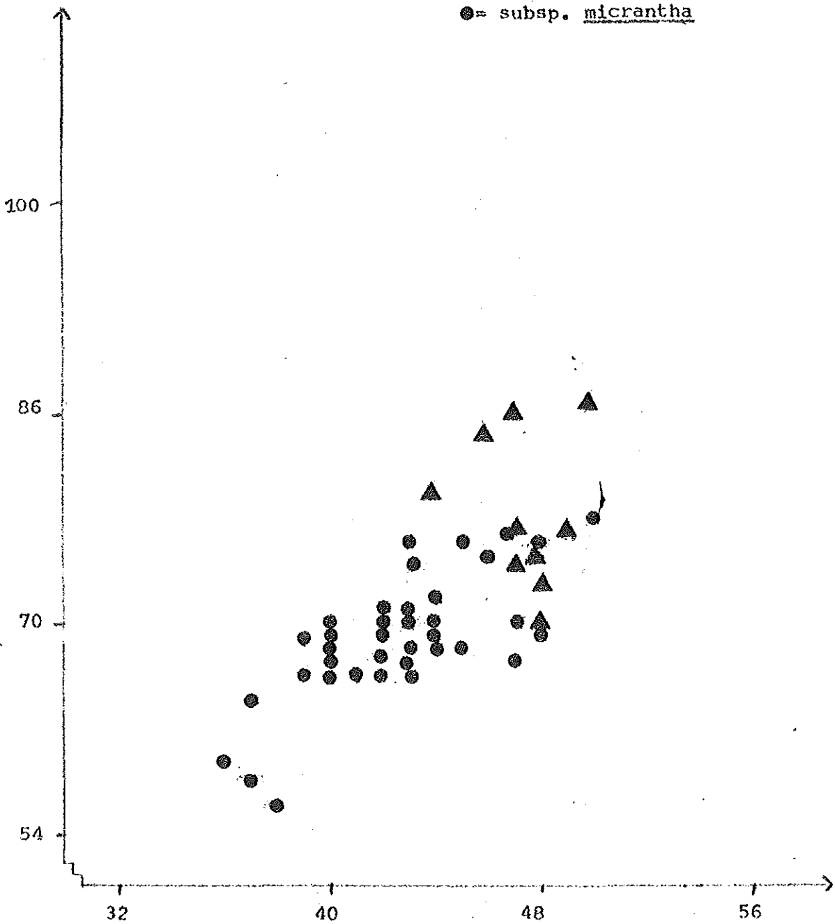
Fig. 23. Scatter diagram illustrating correlation between Equatorial diameter (horizontal axis) and polar axis (vertical axis). Measurements are in \mu\text{m} .
