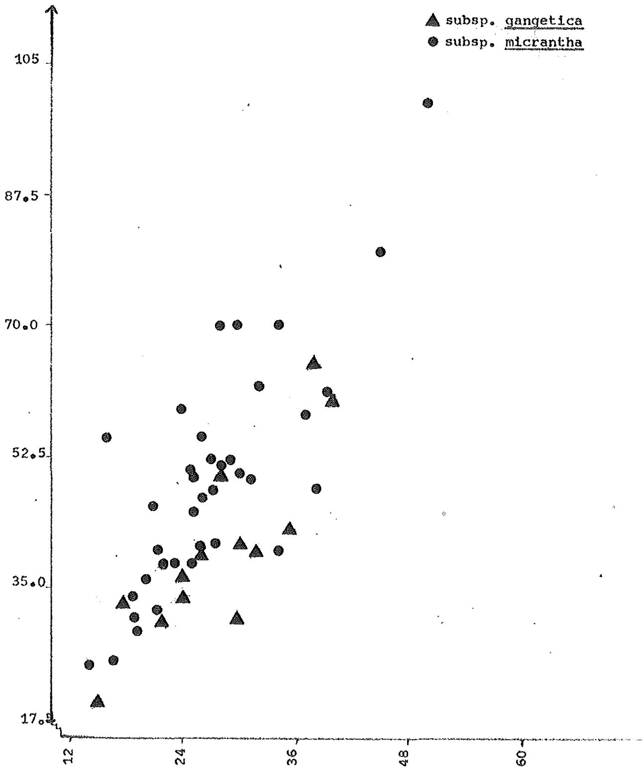
Fig. 16. Scatter diagram illustrating correlation between leaf length (vertical axis) and leaf width (horizontal axis) both in mm. Note : Bullock 2321 is not included.
