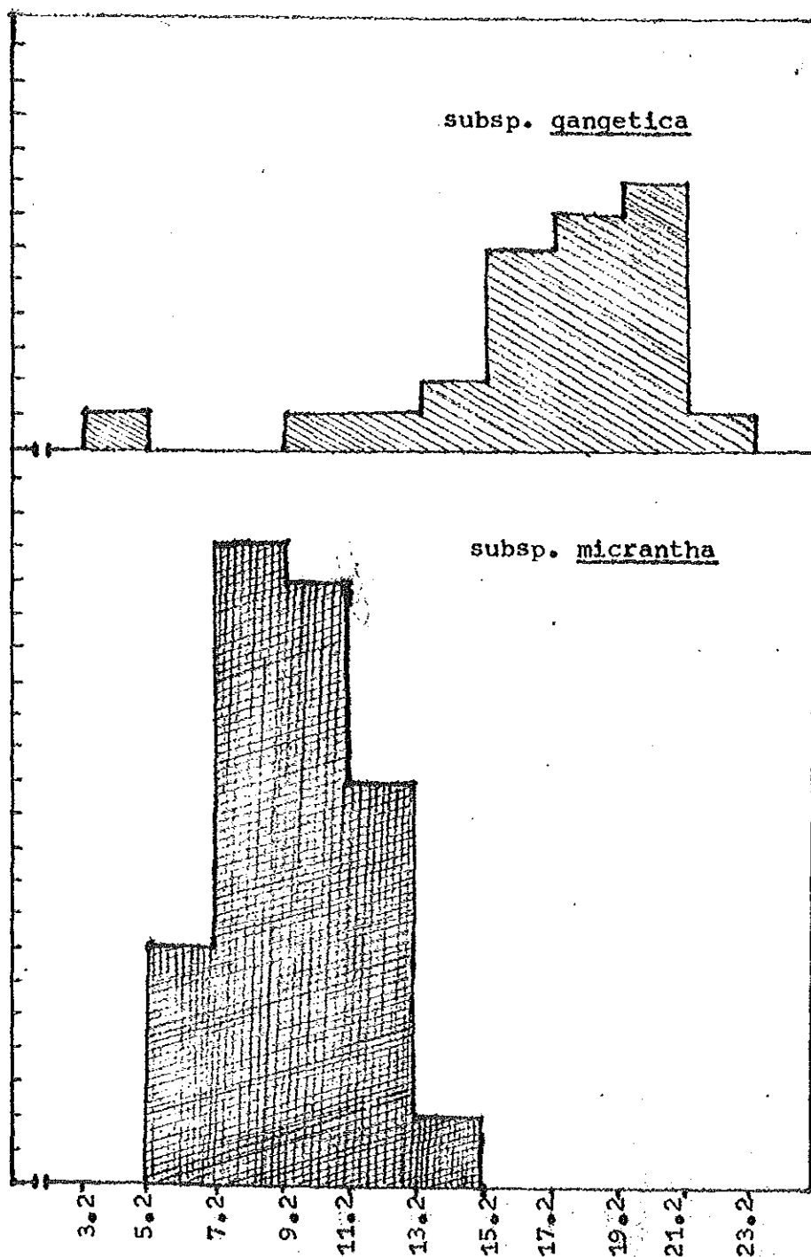
Fig. 19. Histograms illustrating variation in style and stigma length. Horizontal scale shows class intervals for style and stigma length. Vertical all one line represents one collection.
