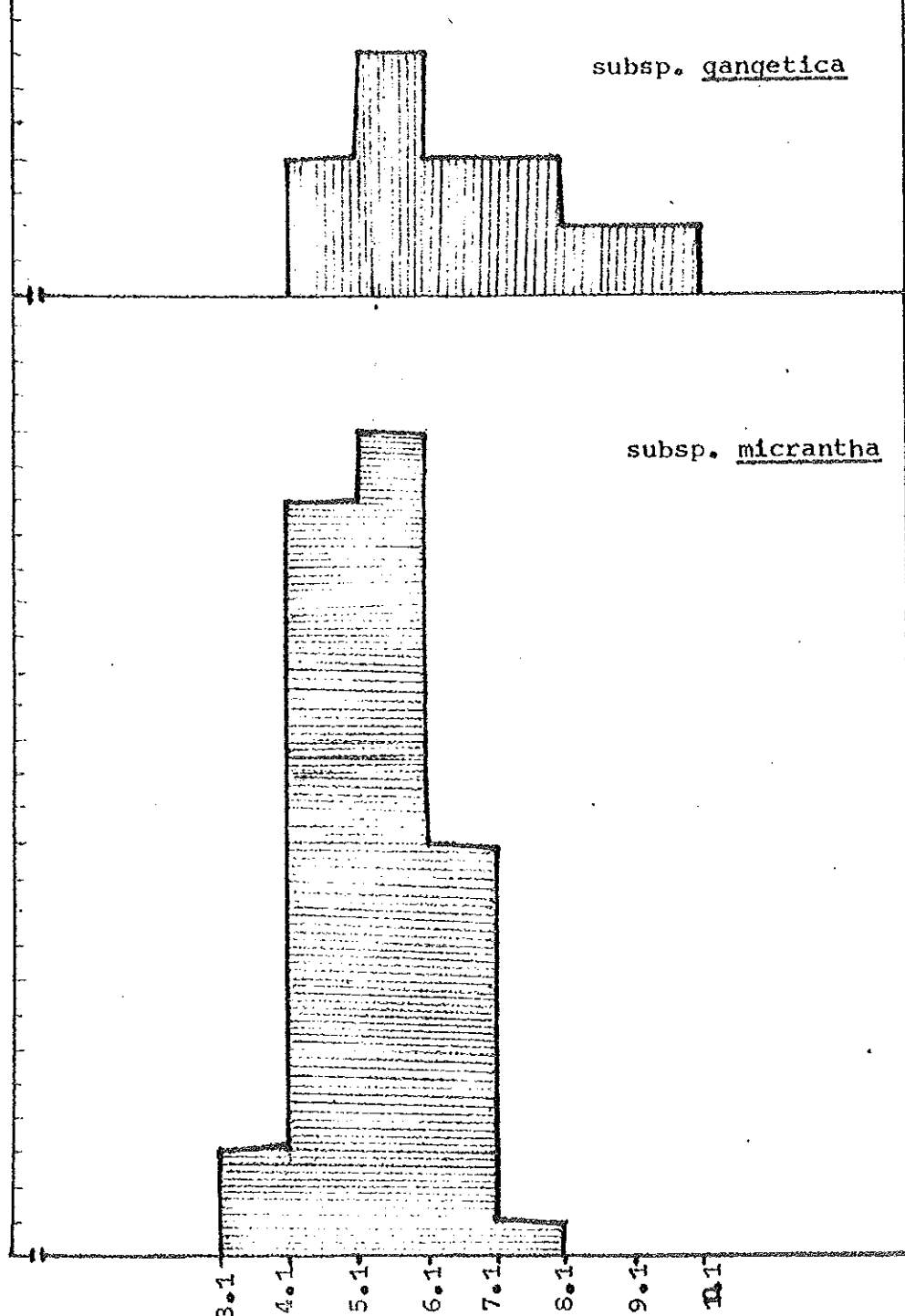
Fig. 17. Histograms illustrating variation in calyx length. Vertically one line represents one collection. Horizontal scale shows class intervals for calyx length.
