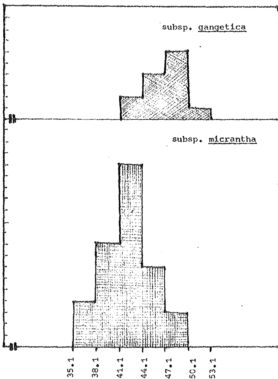
Fig. 22. Histograms illustrating variation in pollen size (Equatorial diameter). Vertically one line represents one collection. Horizontal scale shows class intervals for equatorial diameter.
