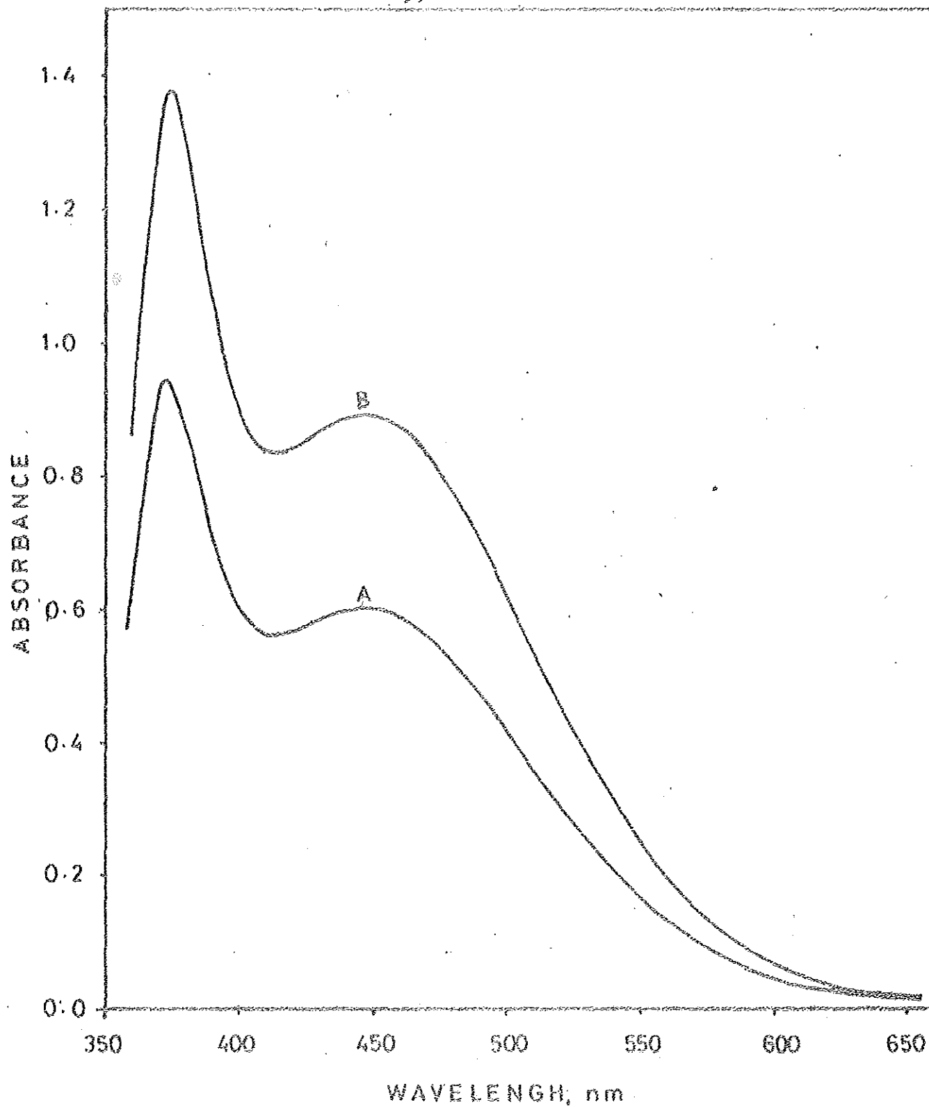
Figure 3 Absorption spectra of (A) 8.0 \times 10^{-5} \text{ M} Fe (III)- \text{N}_3 -PCHA complex (B) 1.2 \times 10^{-4} \text{ M} Fe (III)- \text{N}_3 -PCHA complex against reagent blank in ethylacetate.
