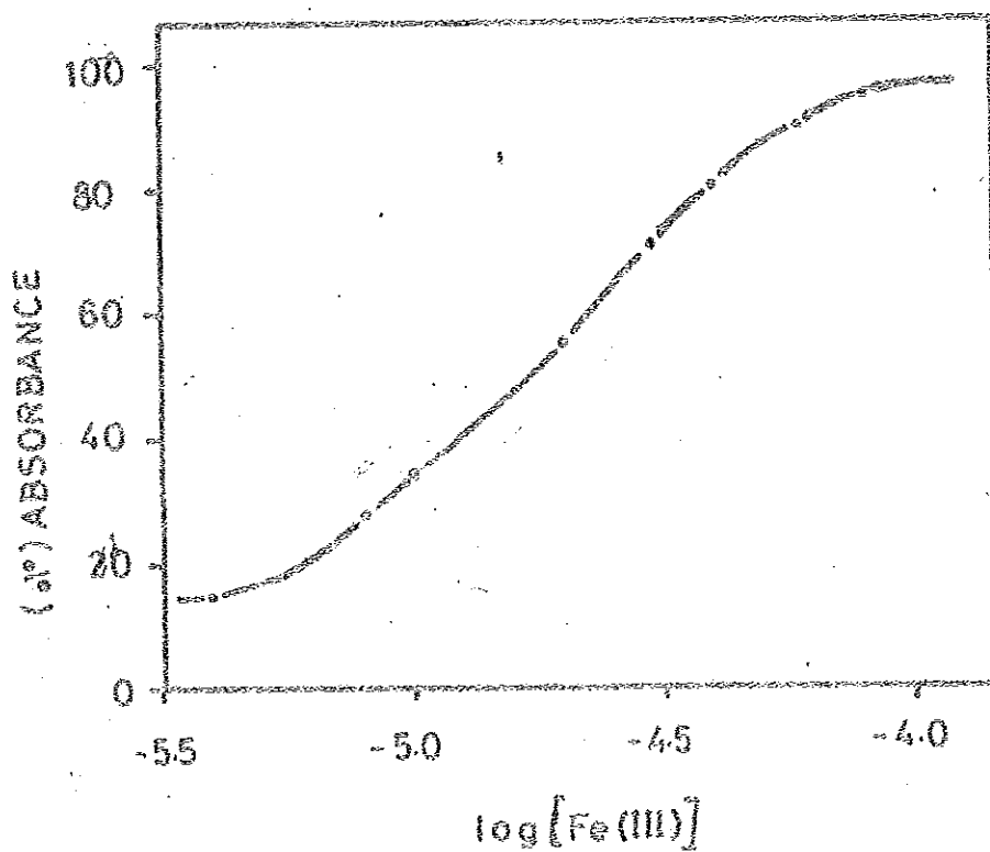
Figure 12 Ringbom's plot for the evaluation of optimum concentration range for determination of Iron(III) by Fe (III)-SCN-PCHA system.
