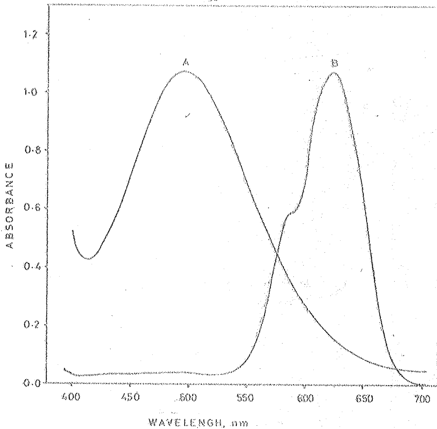
Figure 2 Absorption spectra of (A) 6.0 \times 10^{-5} \text{ M} Fe(III)-SCN-PCNA complex (B) 6.0 \times 10^{-4} \text{ M} Co(II)-SCN complex against reagent blank in ethylacetate.
