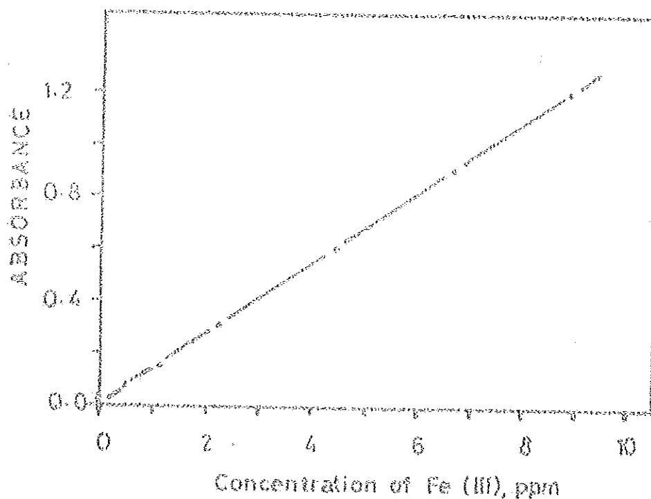
Figure 13 Calibration curve for determination of Iron (III) by Fe(III)-N 3 -PCHA system.
