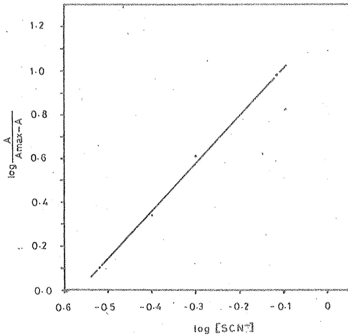
Figure 9. Curve for determination of Iron (III) to \text{SCN}^- ratio in Fe (III) - \text{SCN}^- - PCHA system.
