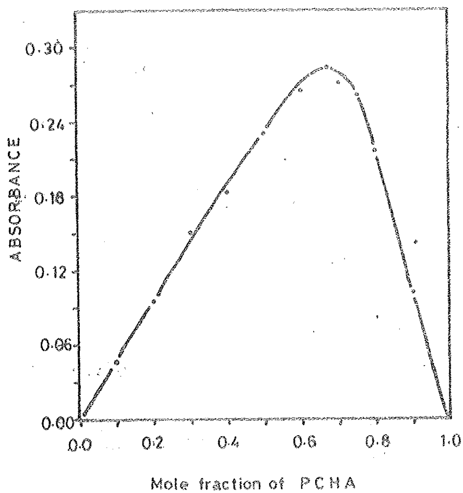
Figure 5 Curve for determination of composition of \text{Fe(III)}-\text{N}_3\text{-PCHA} complex by continuous variations method.
