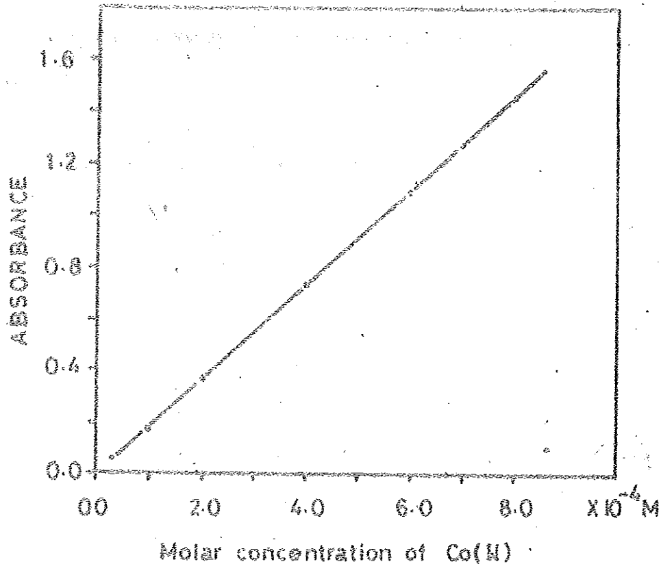
Figure 15 Calibration curve for determination of Cobalt (II).
