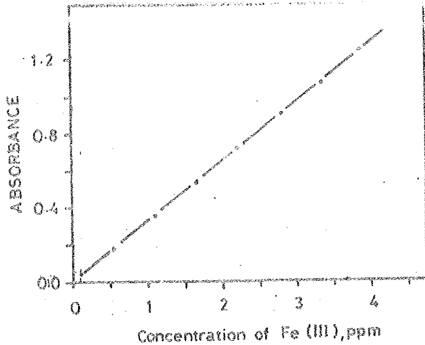
Figure 11 Calibration curve for determination of Iron (III) by Fe (III)-SCN-PCHA system.
