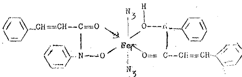
Bis-(N-phenylcinnamohydroxamic acid)diazidoiron(III).
