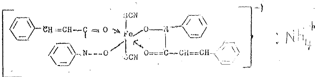
Bis-(N-phenylcinnamohydroxamic acid)dithiocyanatoferrate(III).
