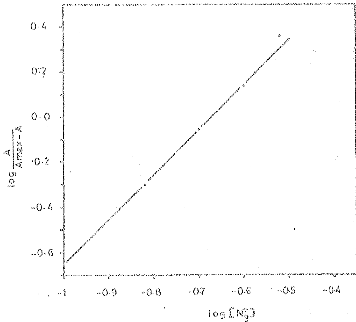
Figure 3 Curve for determination of Iron (III) to N_3^{2+} ratio in Fe (III)- N_3 -PCHA system.
