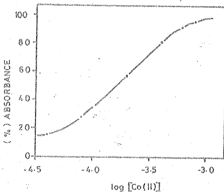
Figure 16 Ringbom's plot for the evaluation of optimum concentration range for determination of Cobalt (II).
