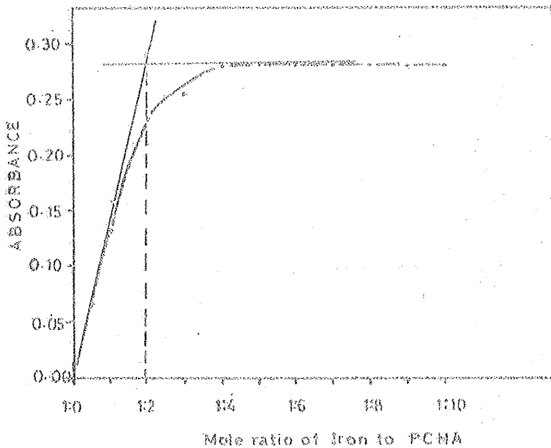
Figure 6. Curve for determination of composition of Fe(III)-SCN-PCHA complex by mole ratio method.
