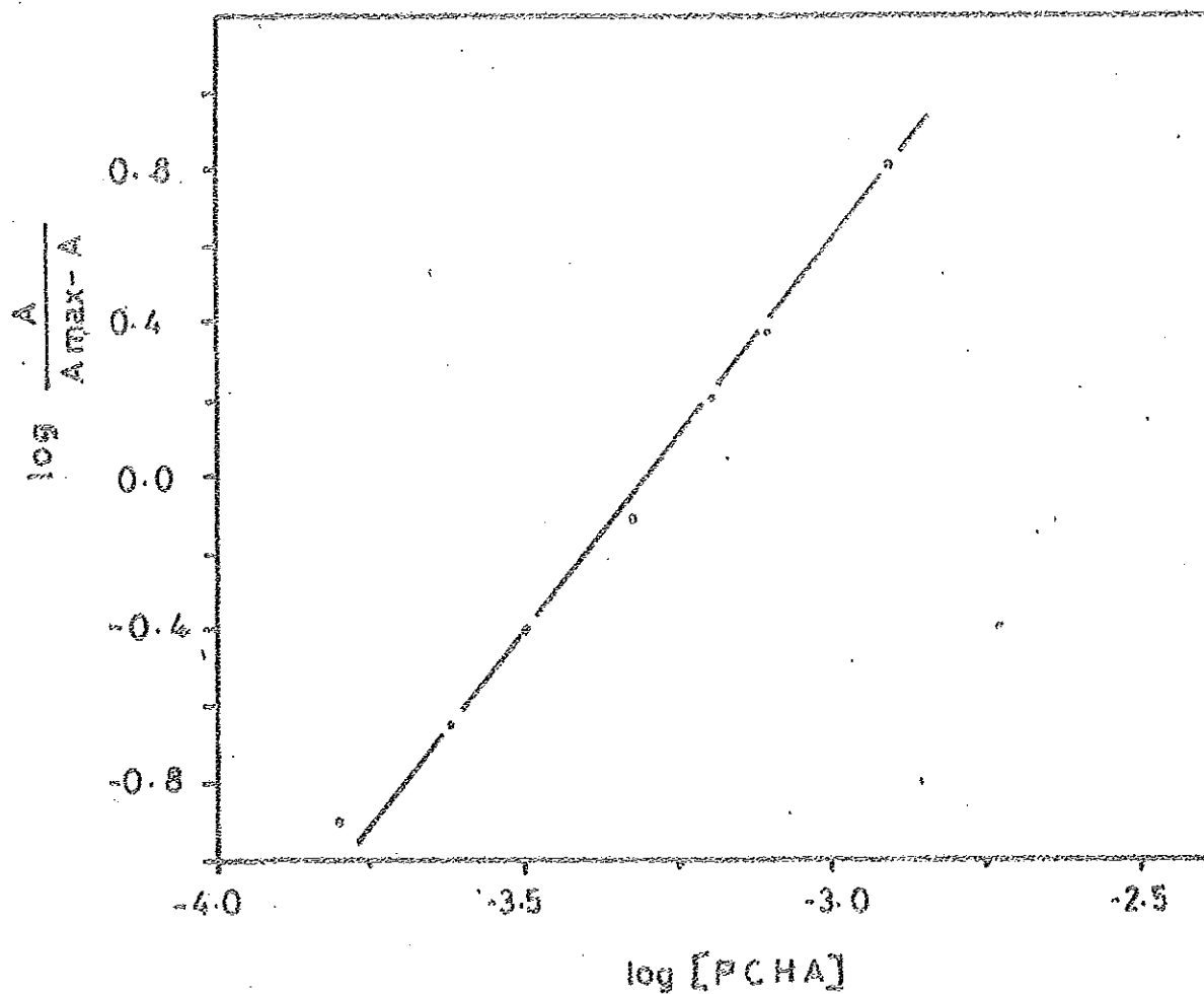
Figure 7. Curve for determination of Iron (III) to PCHA ratio in Fe (III)-N 3 -PCHA system
