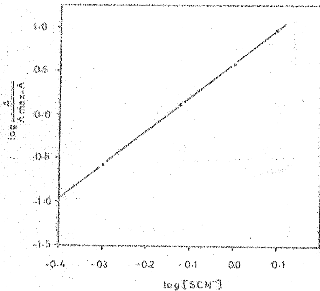
Figure 10 Curve for determination of Cobalt (II) to \text{SCN}^- ratio in \text{Co}(\text{II}) - \text{SCN} system.
