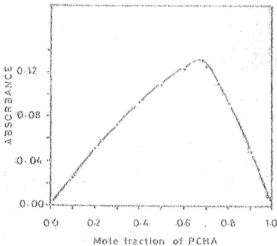
Figure 4 Curve for determination of composition of \text{Fe(III)}\text{-SCN-PCNA} complex by continuous variations method.
