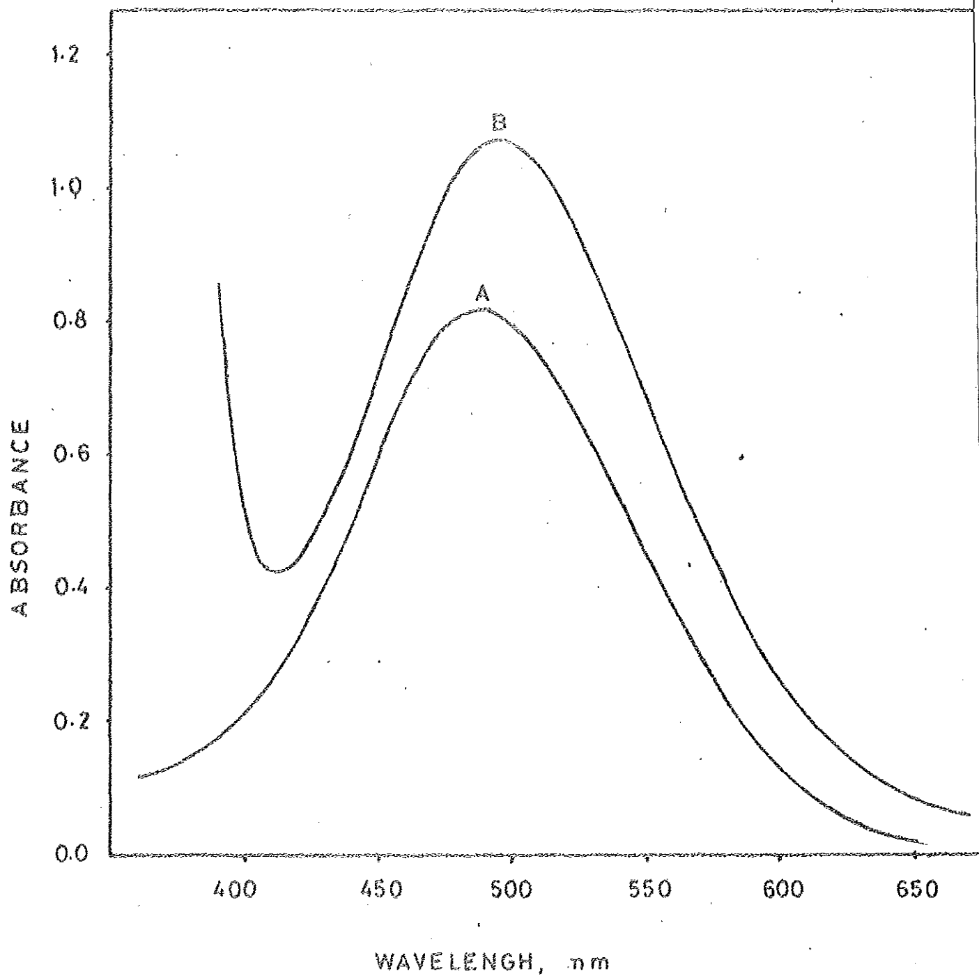
Figure 1. Absorption spectra of (A) 6.0 \times 10^{-5} \text{ M} Fe(III)-SCN complex (B) 6.0 \times 10^{-5} \text{ M} Fe(III)-SCN-PCHA complex against reagent blank in ethylacetate.
