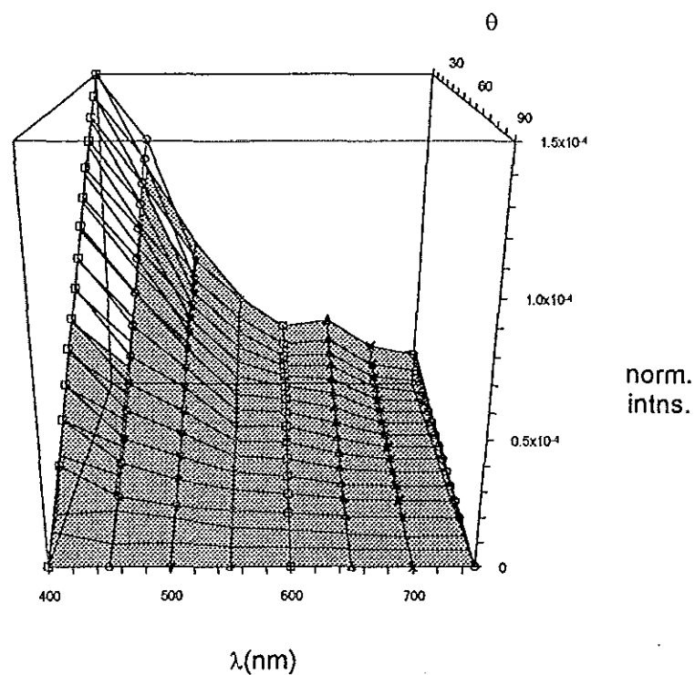
Fig.4.1.8 Three dimensional representaion of normalised intensity as a function of scattering angle \theta and wavelength \lambda for AsahiU. I(\theta, \lambda) = (90-\theta)(a\lambda^2+b\lambda+c) .
