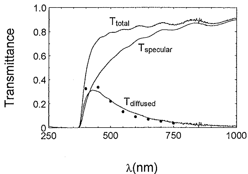
Fig.4.1.10. Specular ,total&diffused transmittances of (20-38)ZnO
