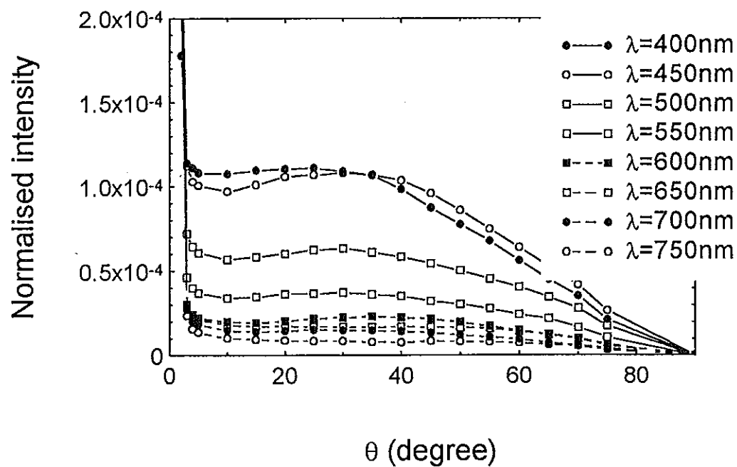
Fig 4.1.11. Angular intensity distribution in transmission for (20-38) ZnO.
