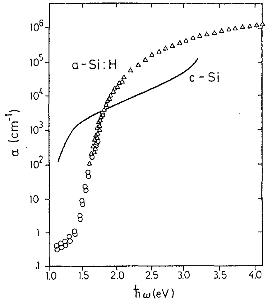
Fig(2.2) Absorption coefficient of a-Si:H derived from optical absorption ( \Delta ) and photoconductivity ( \circ )[13].
