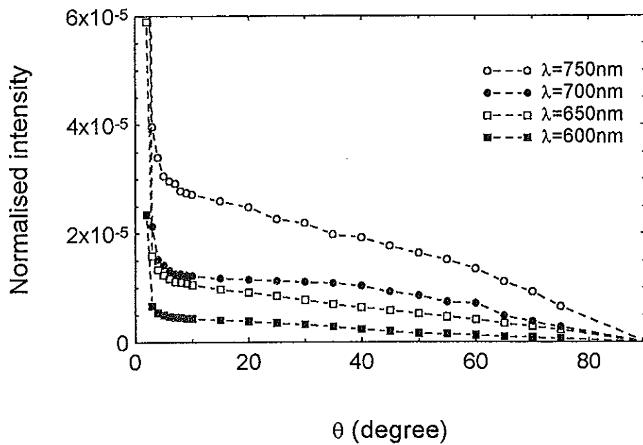
Fig.4.4.6 Angular intensity distribution in transmission for Standard TCO / p-layer (15nm) / i-layer (380nm)
