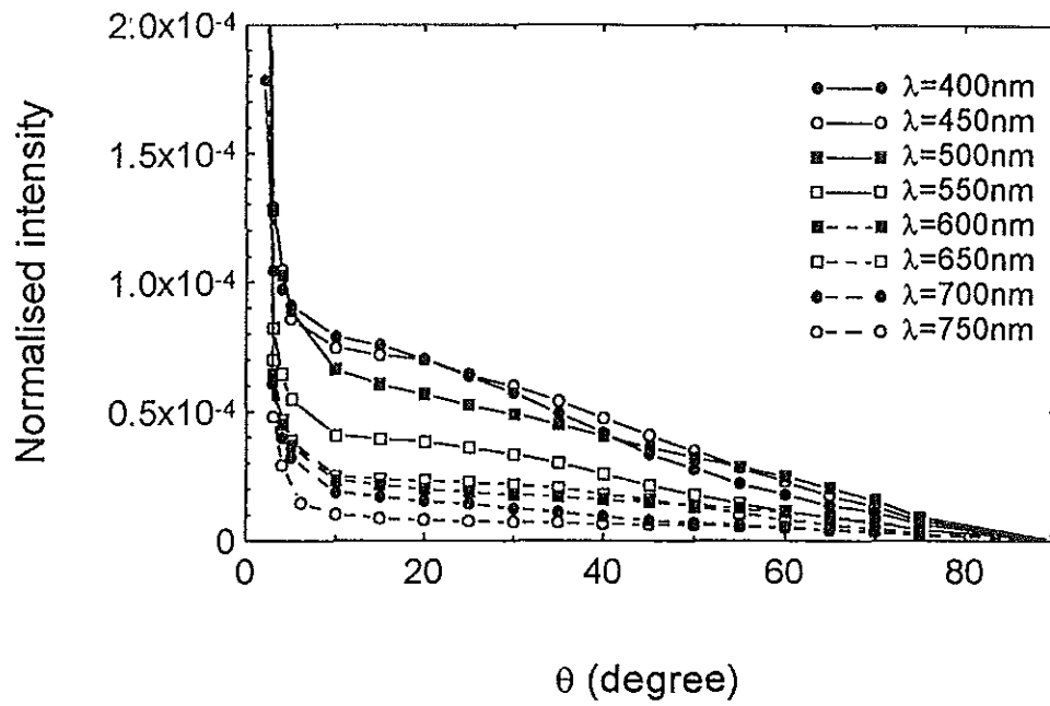
Fig. 4.2.3 Angular intensity distribution in transmission for Asahi U / p-layer (15nm)
