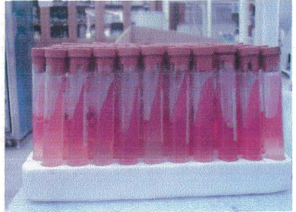
Urease positive
