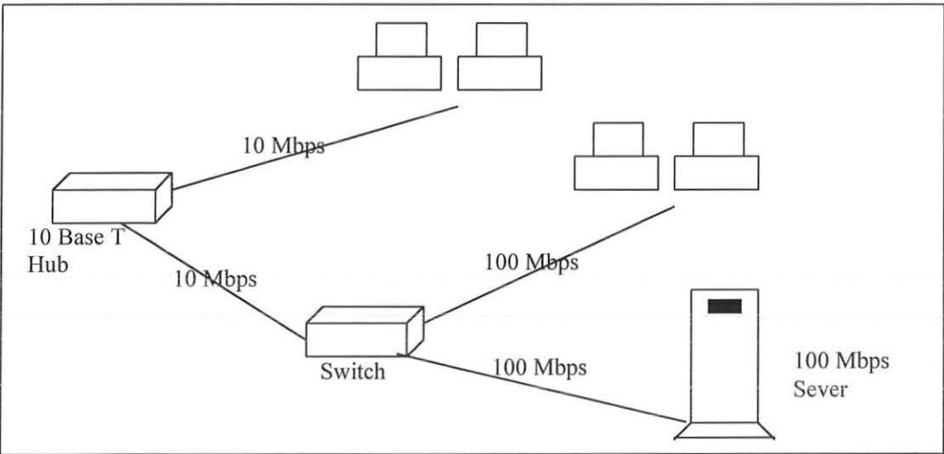
Figure 5-2, Changing the workgroup hubs
