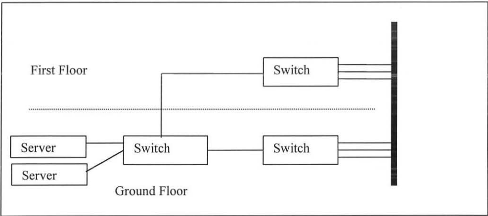
Figure 5-4, Migration at the Backbone
