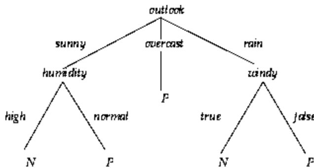
Figure 2.1: Decision tree structure taken from Queens University Belfast, Student Notes [3].
