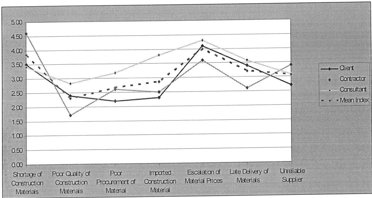
Fig 3.1.1 Scores of material related factors of each group and the relative mean score of all
