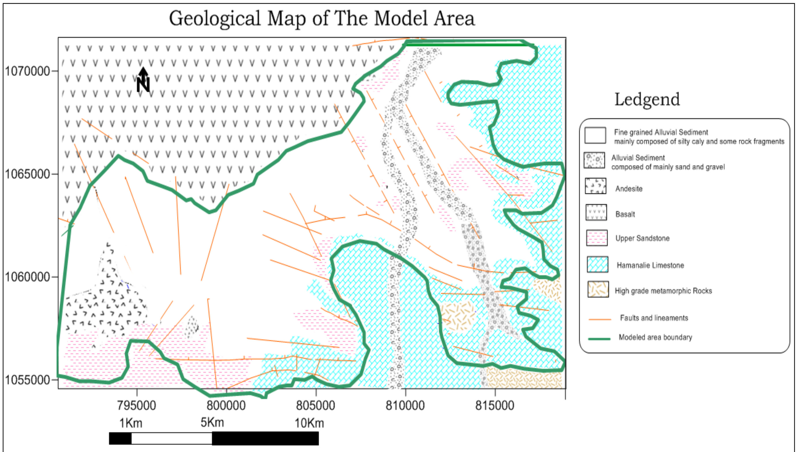
Figure 3: Geological map of the model area modified and simplified from WWDSE, 2004
